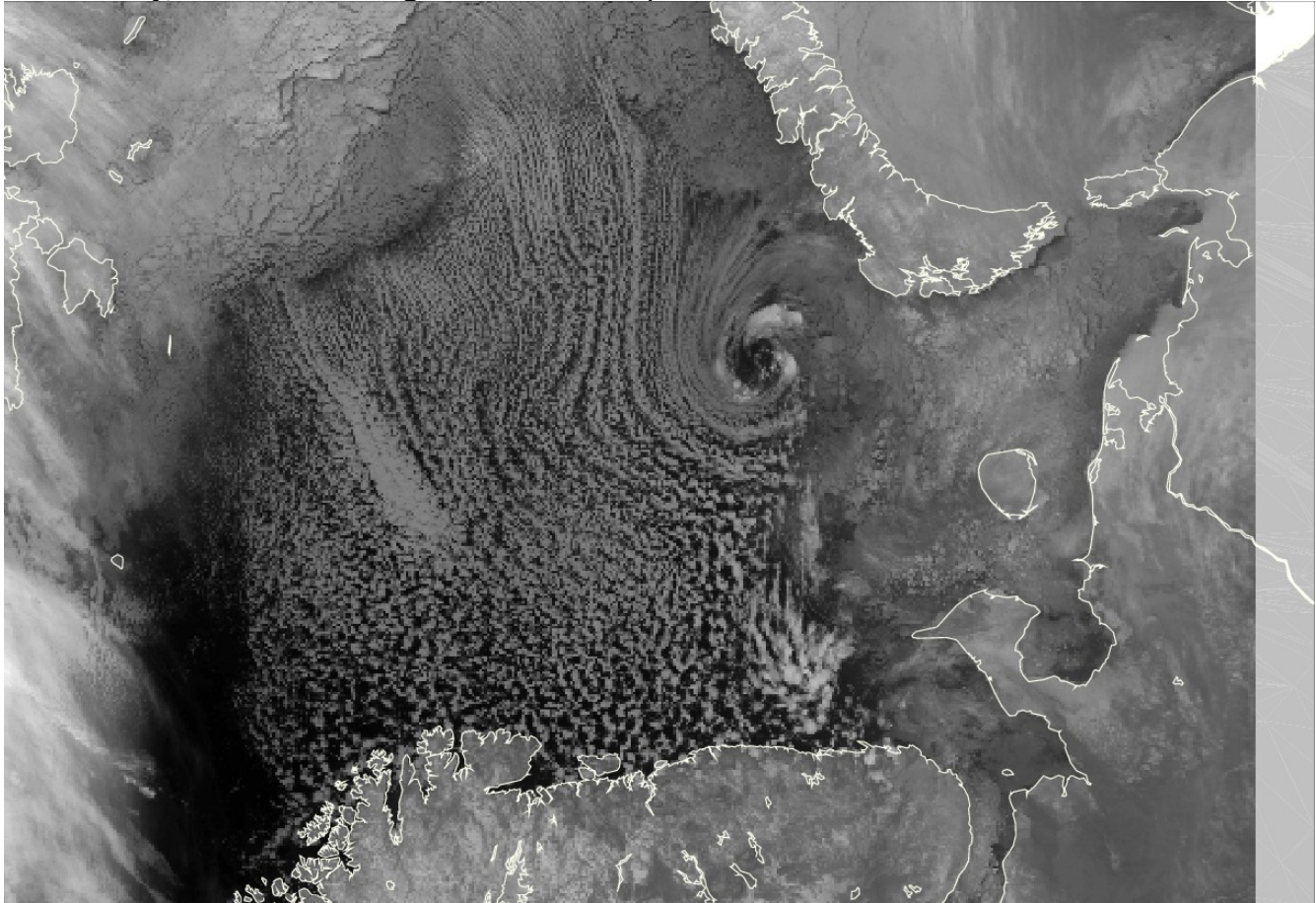
Figure 1: Example of Meso Circulation trailing the ice edge west of Novaya Zemjya 6 March 2010.
