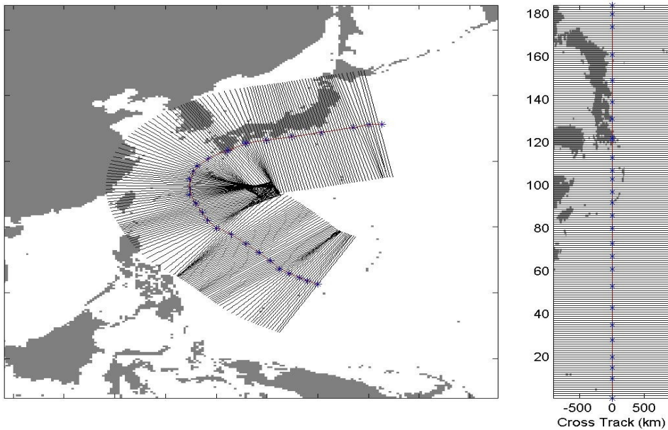
Figure 1: Super Typhoon Man-Yi, 7 – 17 July 2007. The left panel shows the 6-hourly best track positions (blue stars), the interpolated position (red line), and the track orthogonals (black lines) every 25 km. The right panel shows how the evenly spaced orthogonals map onto a grid. Note that the transformation into the storm-centered coordinates does not retain coastlines in a familiar form.
