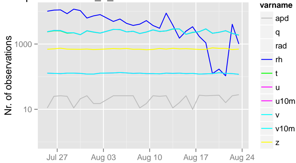
/opdata/arome2_5_main/ccma/ts/ccma.db 12 UTC
