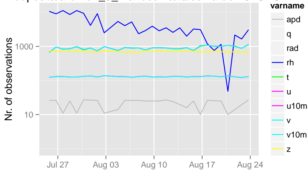
/opdata/arome2_5_main/ccma/ts/ccma.db 18 UTC
