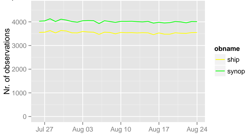
/opdata/arome2_5_main/ecma_sfc/ts/ecma.db 00 UTC
