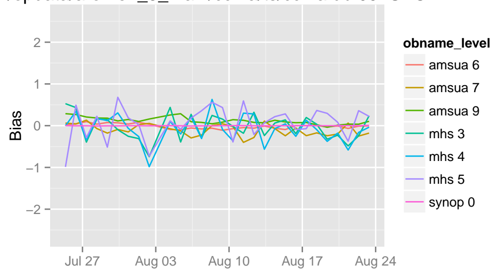
/opdata/arome2_5_main/ccma/ts/ccma.db 09 UTC
