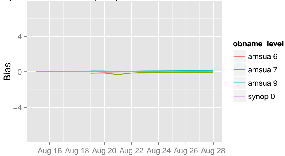
/opdata/arome2_5_preop/ccma/ts/ccma.db 00 UTC
