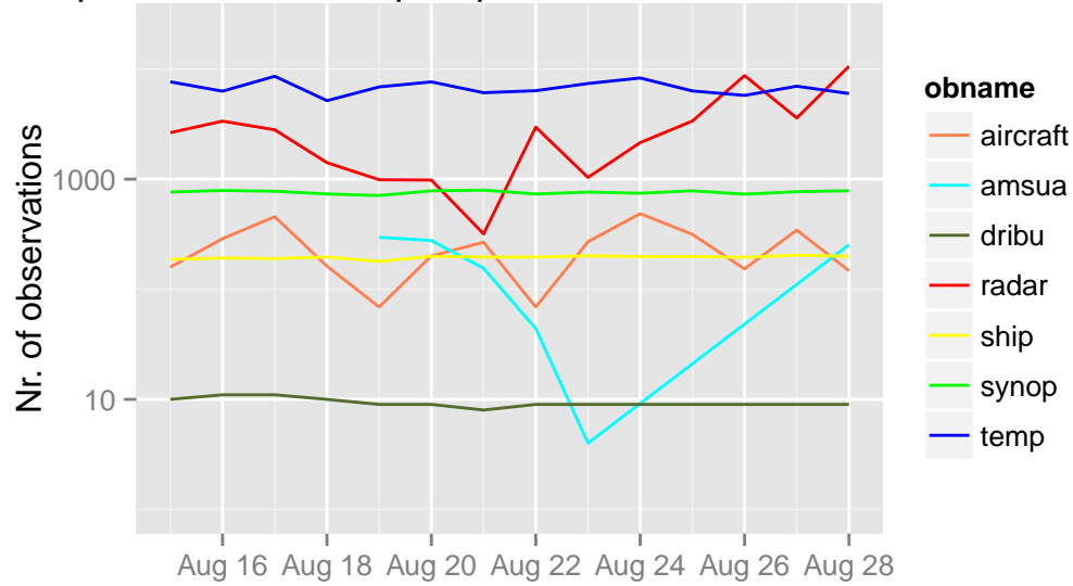
/opdata/arome2_5_preop/ccma/ts/ccma.db 00 UTC
