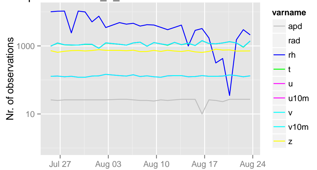
/opdata/arome2_5_main/ccma/ts/ccma.db 15 UTC
