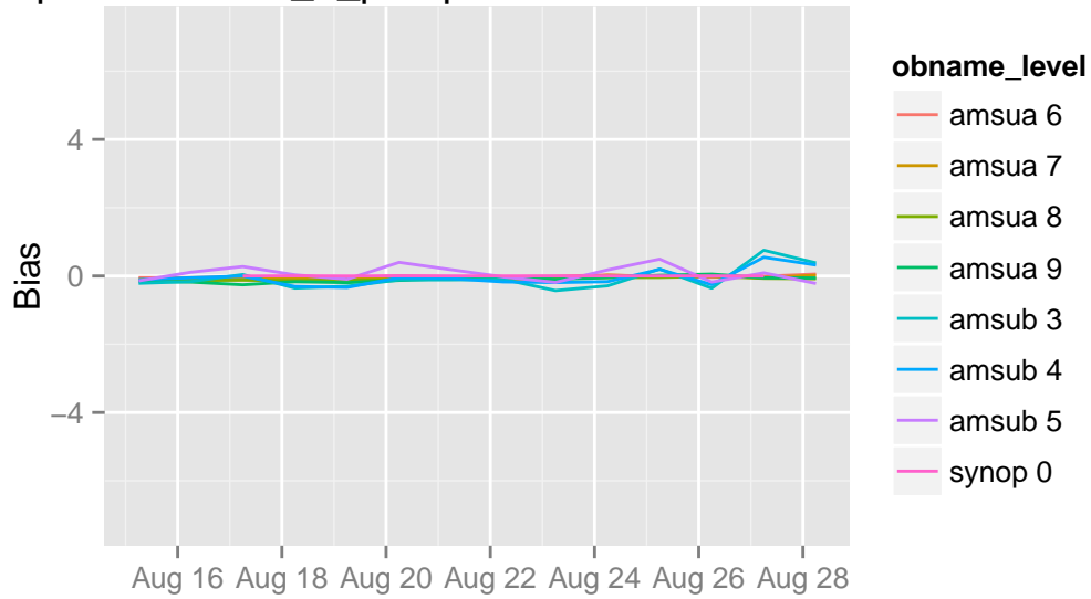
/opdata/arome2_5_preop/ccma/ts/ccma.db 06 UTC
