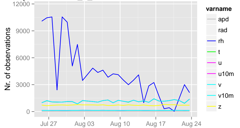
/opdata/arome2_5_main/ccma/ts/ccma.db 15 UTC
