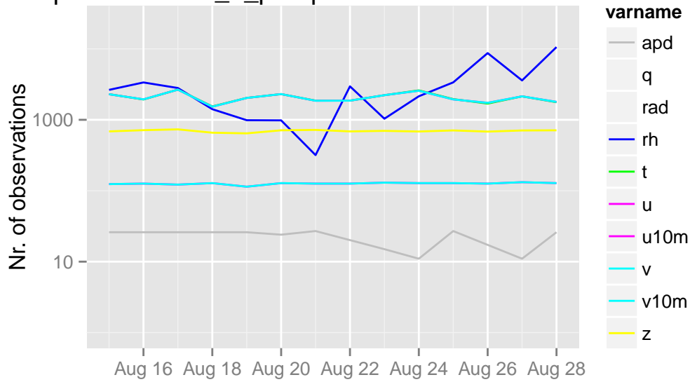
/opdata/arome2_5_preop/ccma/ts/ccma.db 00 UTC
