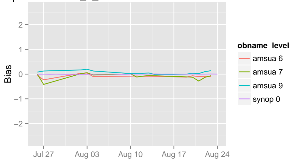
/opdata/arome2_5_main/ccma/ts/ccma.db 00 UTC
