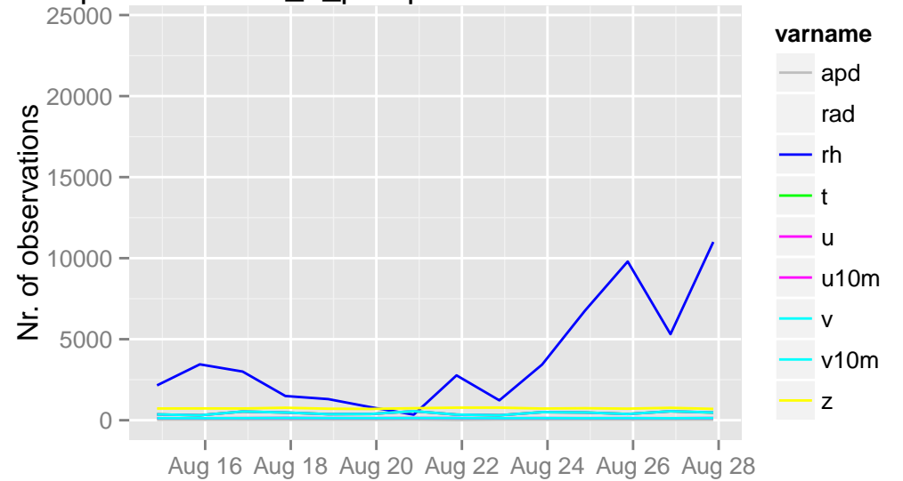
/opdata/arome2_5_preop/ccma/ts/ccma.db 21 UTC
