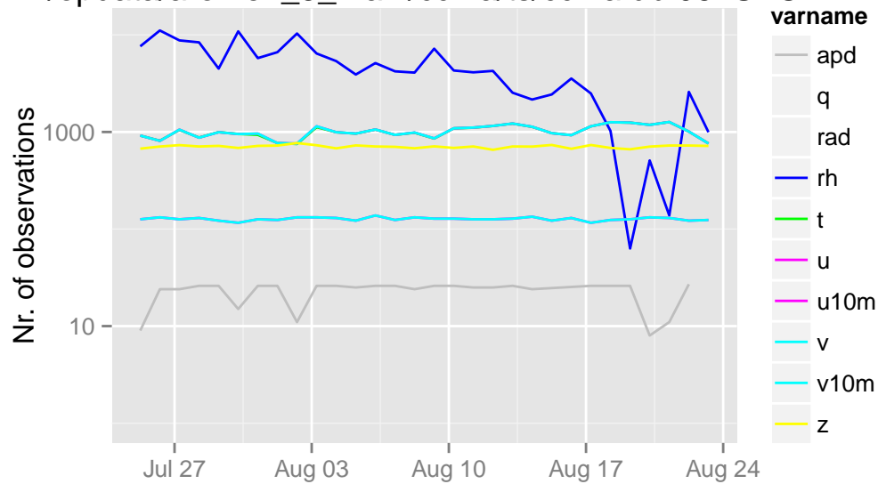
/opdata/arome2_5_main/ccma/ts/ccma.db 06 UTC
