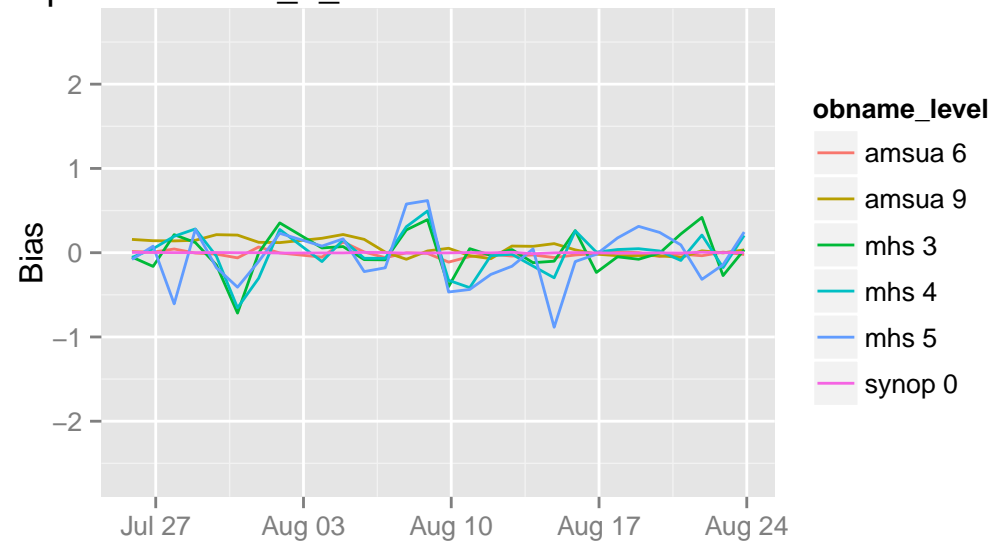
/opdata/arome2_5_main/ccma/ts/ccma.db 21 UTC
