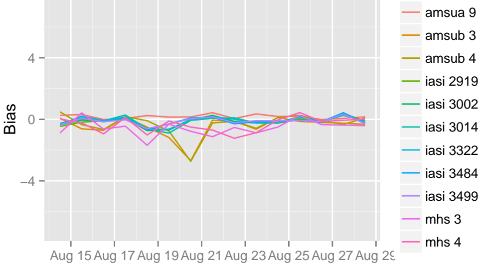
/opdata/arome2_5_preop/ccma/ts/ccma.db 12 UTC
