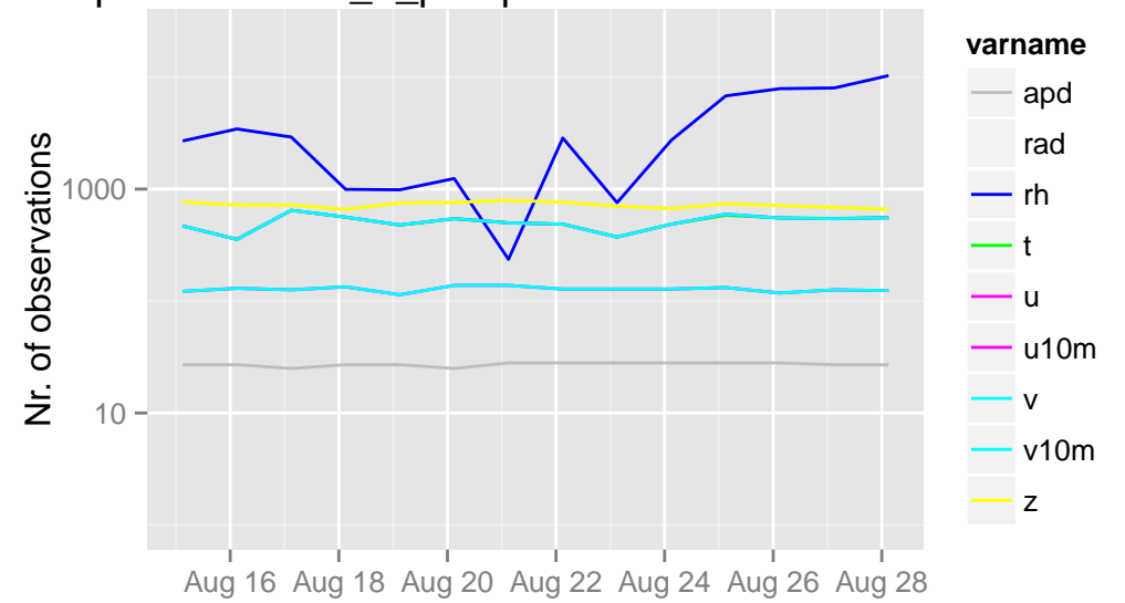
/opdata/arome2_5_preop/ccma/ts/ccma.db 03 UTC
