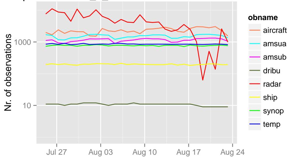
/opdata/arome2_5_main/ccma/ts/ccma.db 06 UTC
