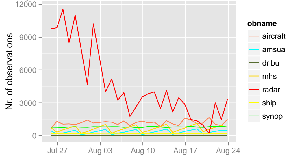
/opdata/arome2_5_main/ccma/ts/ccma.db 21 UTC
