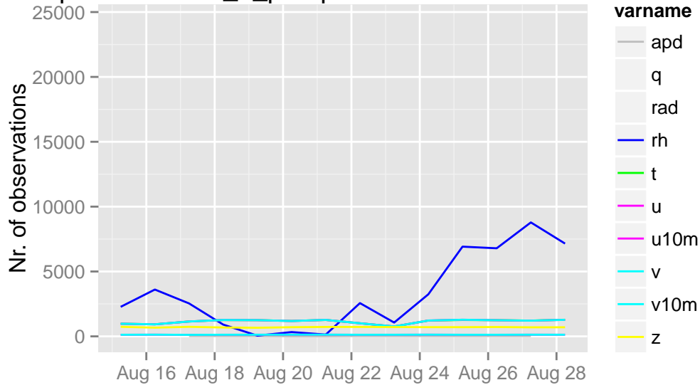
/opdata/arome2_5_preop/ccma/ts/ccma.db 06 UTC
