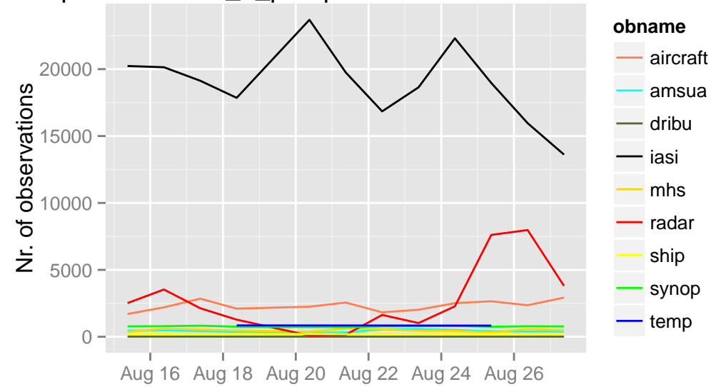
/opdata/arome2_5_preop/ccma/ts/ccma.db 09 UTC
