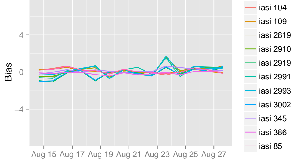
/opdata/arome2_5_preop/ccma/ts/ccma.db 15 UTC
