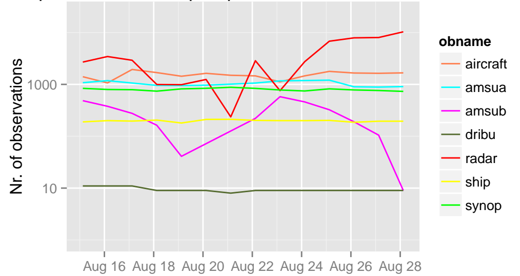
/opdata/arome2_5_preop/ccma/ts/ccma.db 03 UTC
