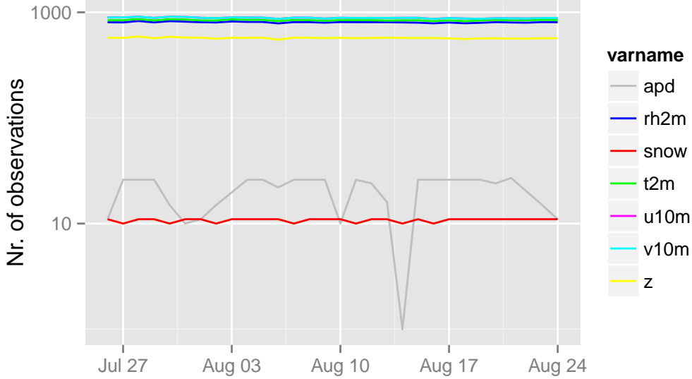
/opdata/arome2_5_main/ecma_sfc/ts/ecma.db 00 UTC
