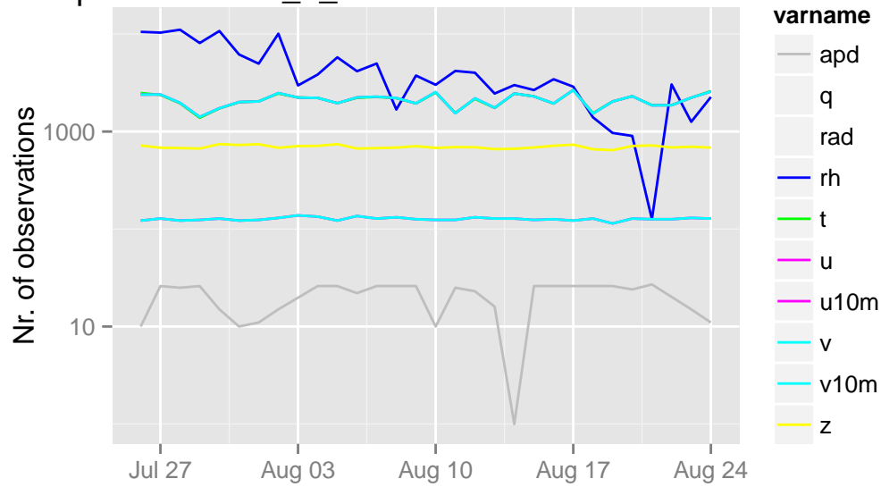
/opdata/arome2_5_main/ccma/ts/ccma.db 00 UTC
