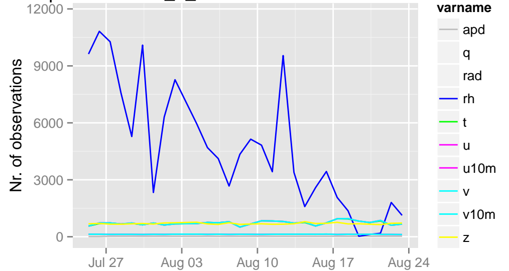
/opdata/arome2_5_main/ccma/ts/ccma.db 09 UTC
