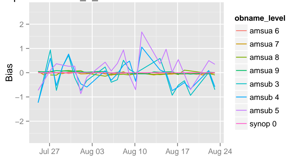
/opdata/arome2_5_main/ccma/ts/ccma.db 03 UTC
