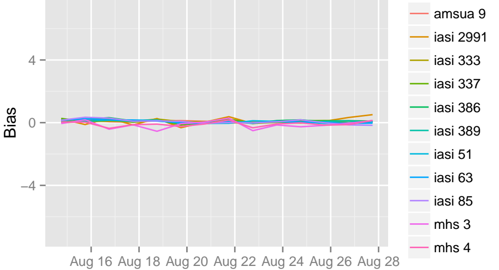
/opdata/arome2_5_preop/ccma/ts/ccma.db 18 UTC
