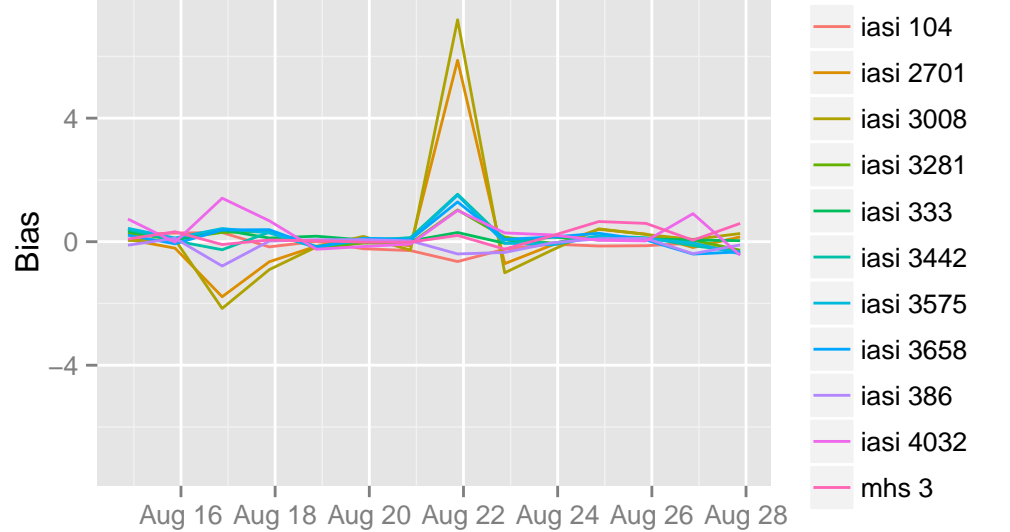
/opdata/arome2_5_preop/ccma/ts/ccma.db 21 UTC
