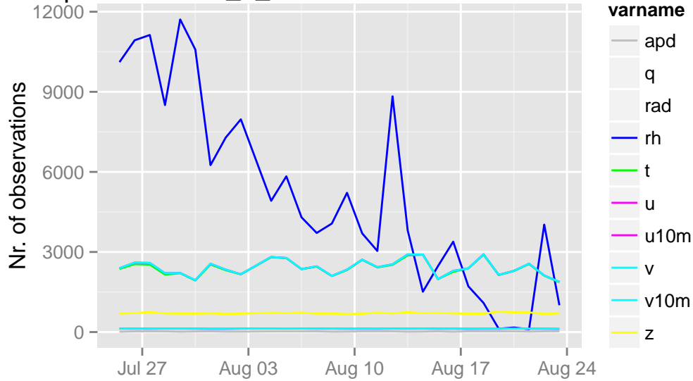
/opdata/arome2_5_main/ccma/ts/ccma.db 12 UTC
