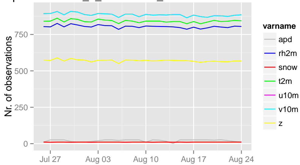
/opdata/arome2_5_main/ecma_sfc/ts/ecma.db 00 UTC
