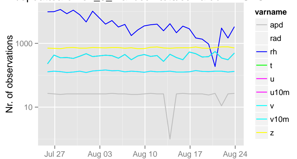
/opdata/arome2_5_main/ccma/ts/ccma.db 21 UTC
