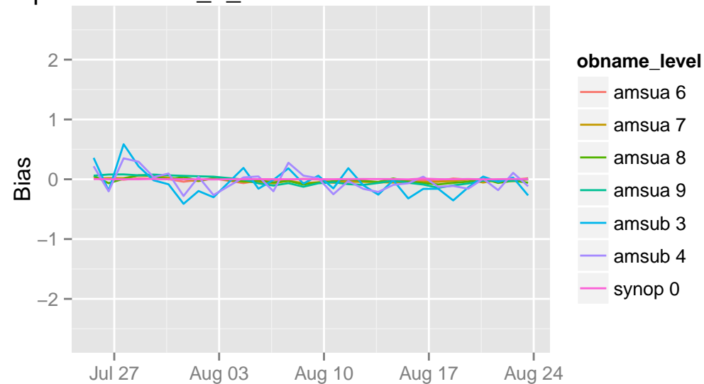
/opdata/arome2_5_main/ccma/ts/ccma.db 15 UTC
