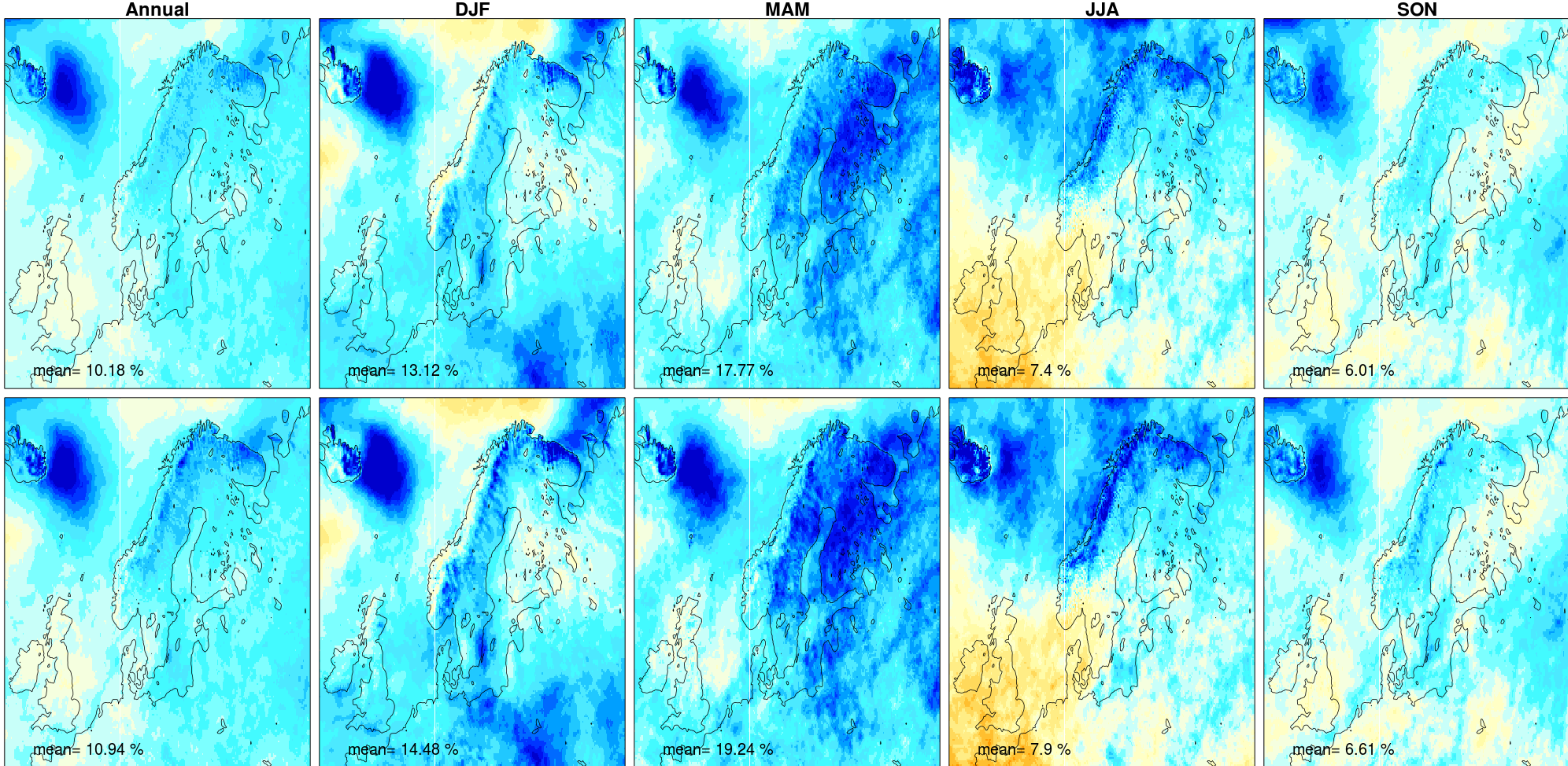
Rel. precipitation change (2071-2100 (RCP4.5) vs. 1971-2000) [%] | Top: Raw | Bottom: Bias-corrected (METNO-QMAP-MESAN-1989-2010)
