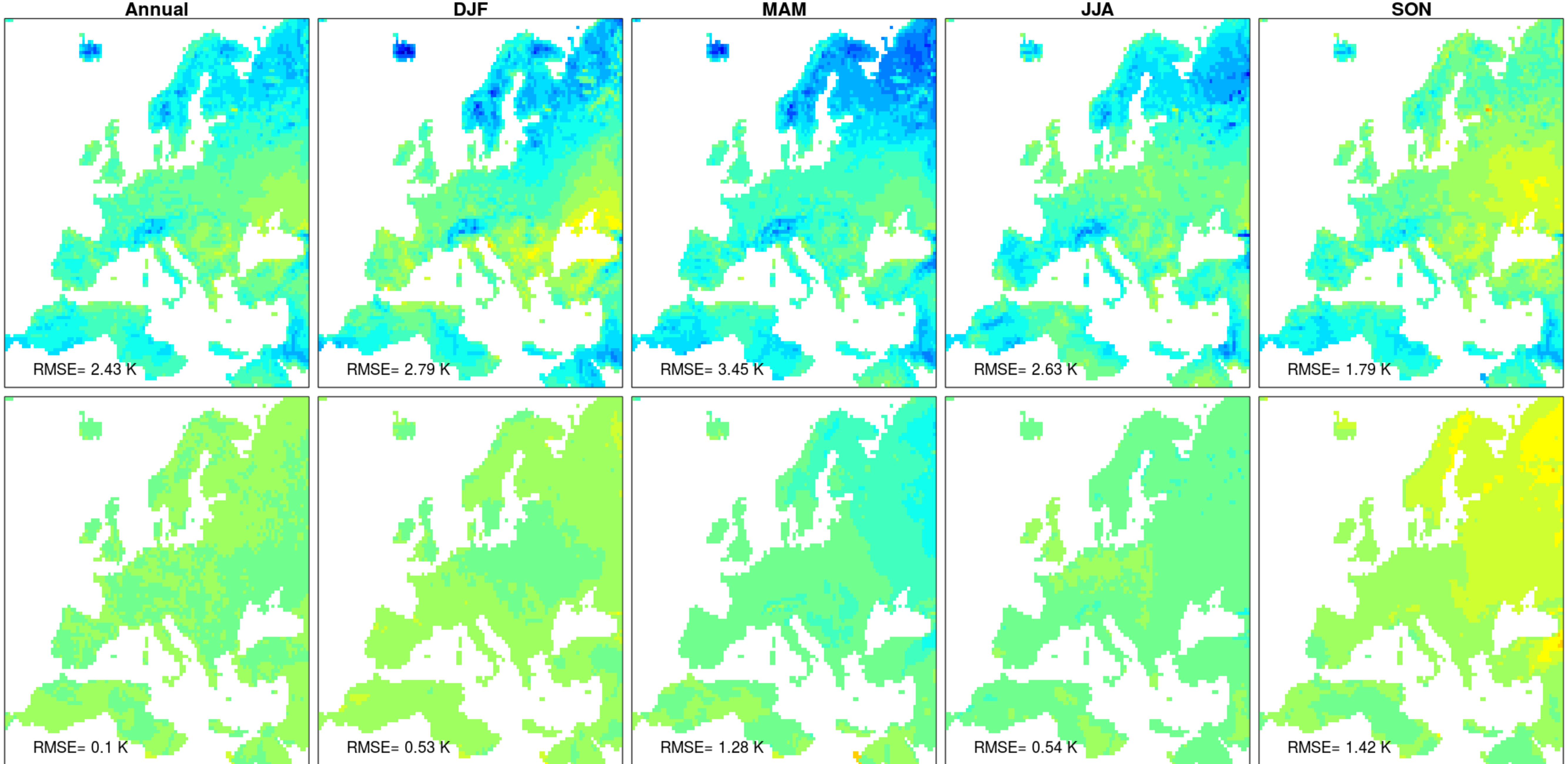
Min. daily temperature bias [K] | Top: Raw | Bottom: Bias-corrected (METNO-QMAP-EOBS10-1981-2010)
