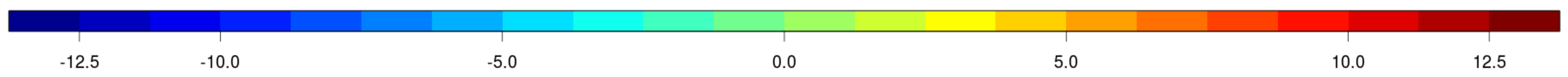
Min. daily temperature bias [K] | Top: Raw | Bottom: Bias-corrected (METNO-QMAP-EOBS10-1981-2010)
