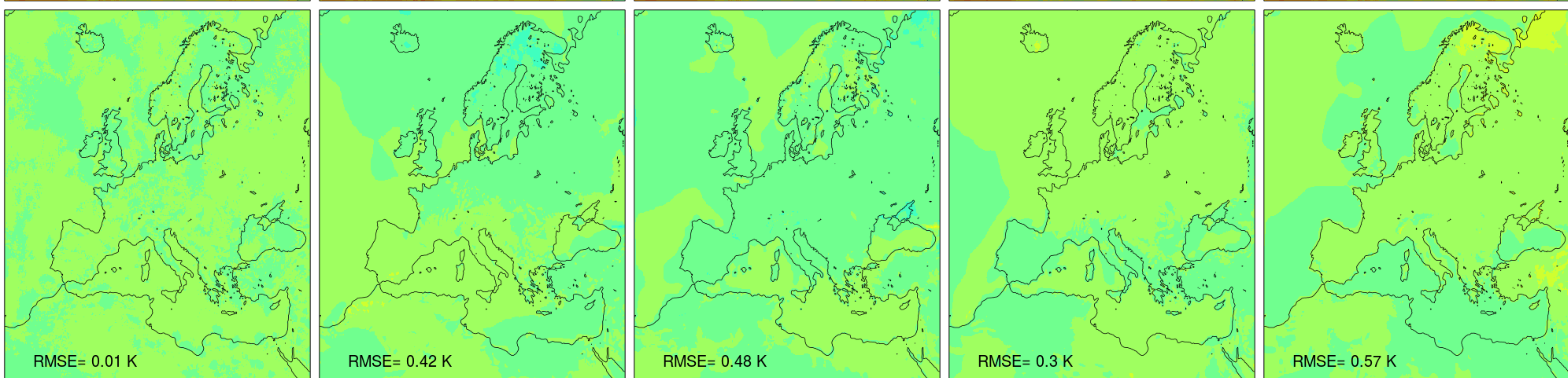
Min. daily temperature bias [K] | Top: Raw | Bottom: Bias-corrected (METNO-QMAP-MESAN-1989-2010)
