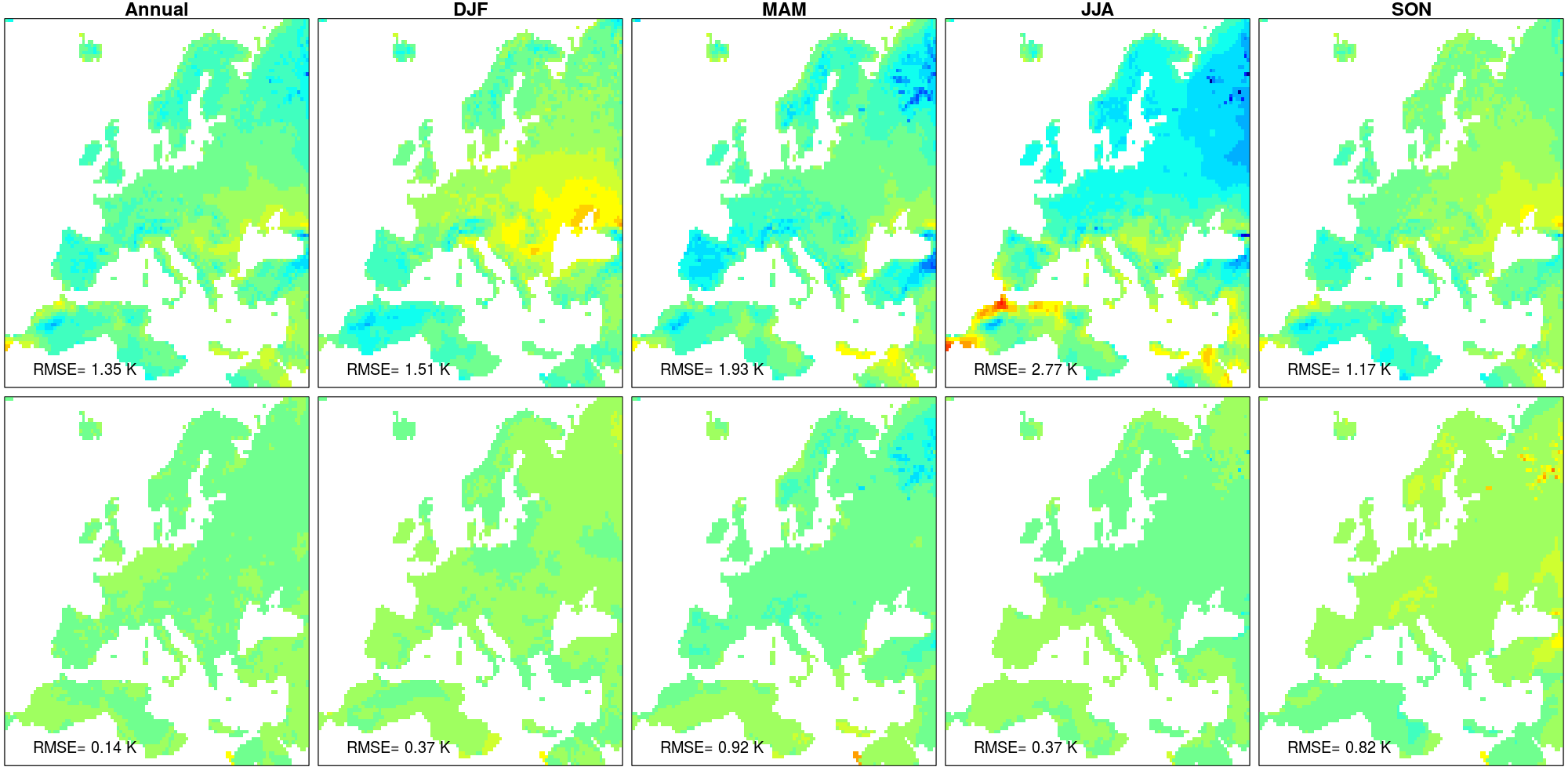
Max. daily temperature bias [K] | Top: Raw | Bottom: Bias-corrected (METNO-QMAP-EOBS10-1981-2010)
