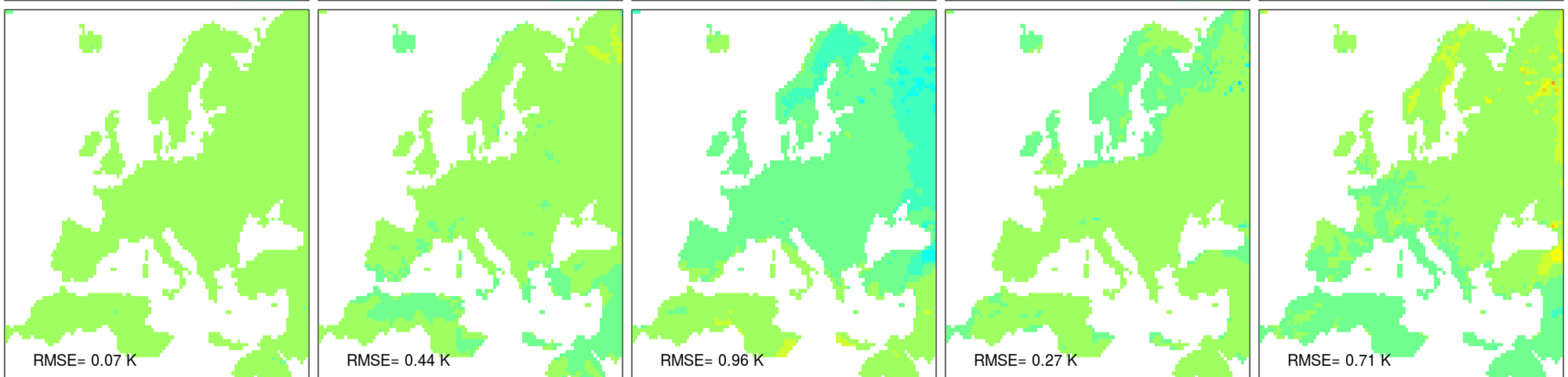
Temperature bias [K] | Top: Raw | Bottom: Bias-corrected (METNO-QMAP-EOBS10-1981-2010)
