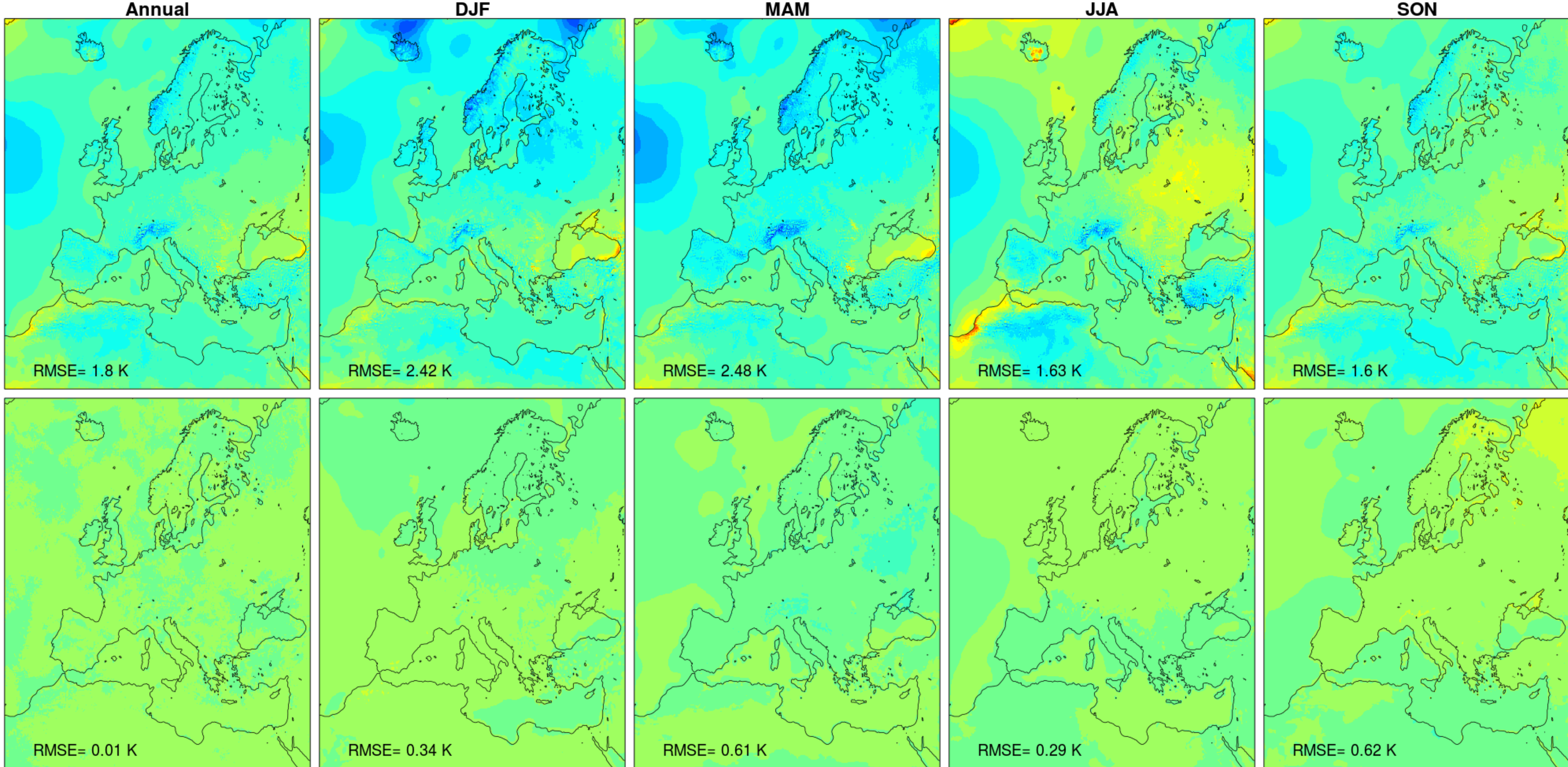
Temperature bias [K] | Top: Raw | Bottom: Bias-corrected (METNO-QMAP-MESAN-1989-2010)
